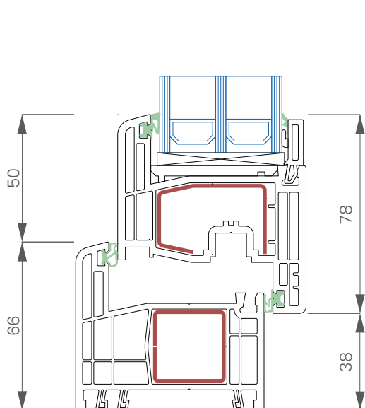
Vertical cross-section
