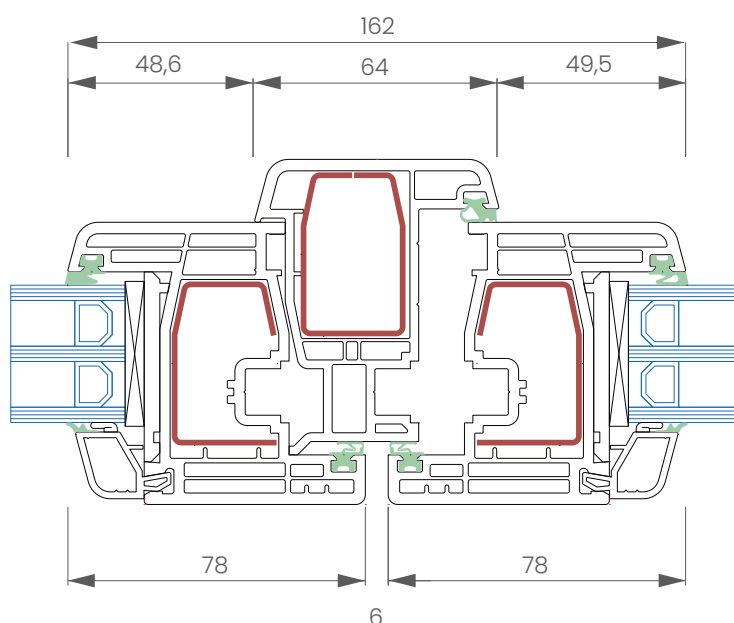
Horizontal cross-section
