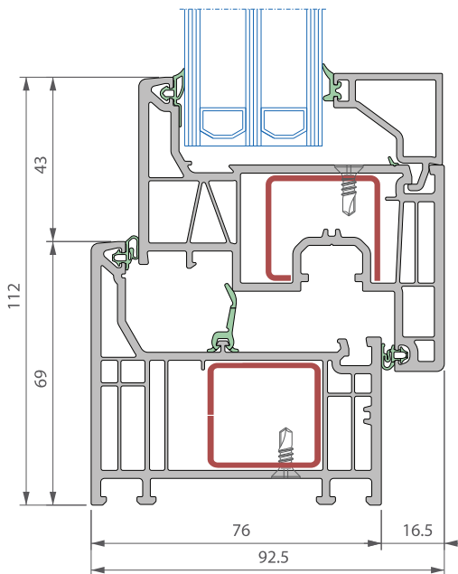
Vertical cross-section
