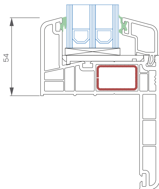
Section verticale
